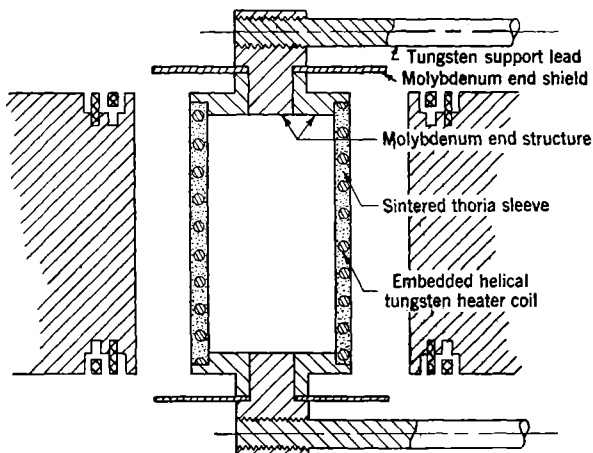
FIG. 12-26.—Thorium oxide cathode of the 4J70. (2 X.)
